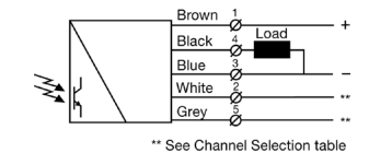
SMR 9XX0 Transistor PNP
