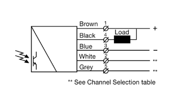
SMR 9XX0 Transistor NPN
